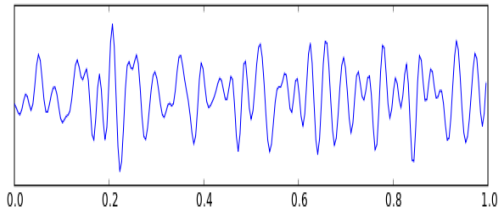
Figure 6 Beta waves
