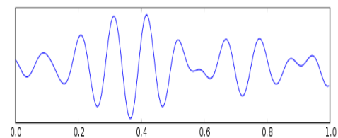
Figure 5 Alpha waves
