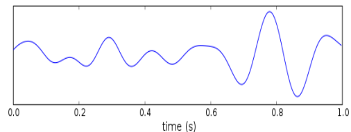
Figure 4 Theta waves
