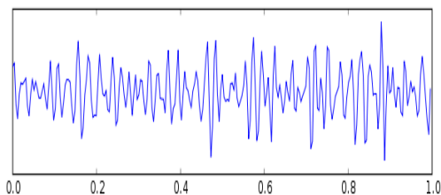
Figure 7 Gamma waves
